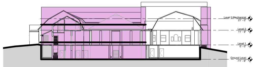
1 Cross Section - East/West - Option 1 1/16" = 1'-0"
