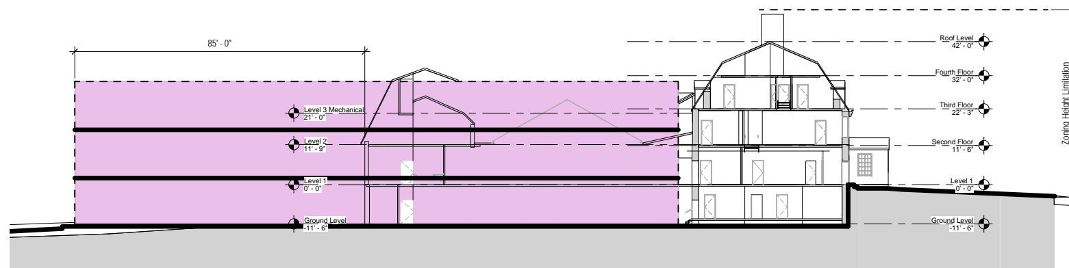
2 Longitudinal Section - North/South - Option 1 1/16" = 1'-0"
