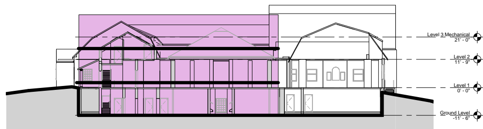
3 Cross Section - East/West Option 2 1/16" = 1'-0"
